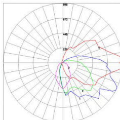
SEE ROAD REPORT! PHOTOMETRIC FILENAME: LM1041.RT8 POLAR GRAPH
